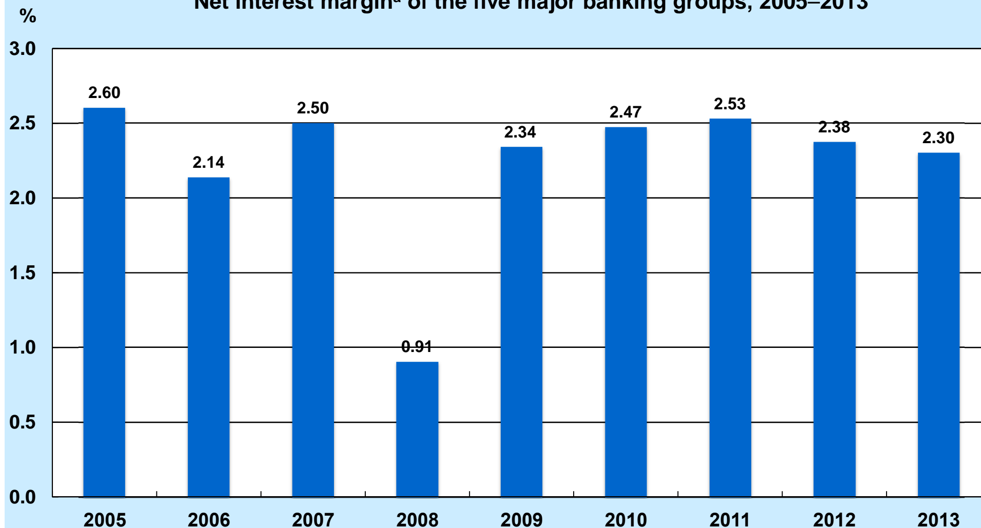
Figure 1.26 Net interest margin a of the five major banking groups, 2005–2013
